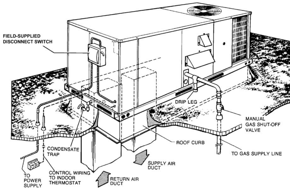
FIGURE 9 - TYPICAL APPLICATIONS
