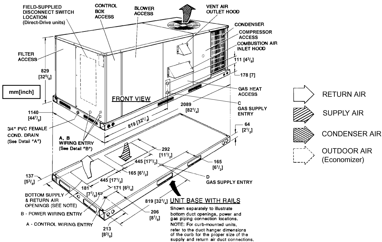
FIGURE 4 - UNIT DIMENSIONS (3 - 6 TON COOLING/GAS HEAT) FRONT VIEW
