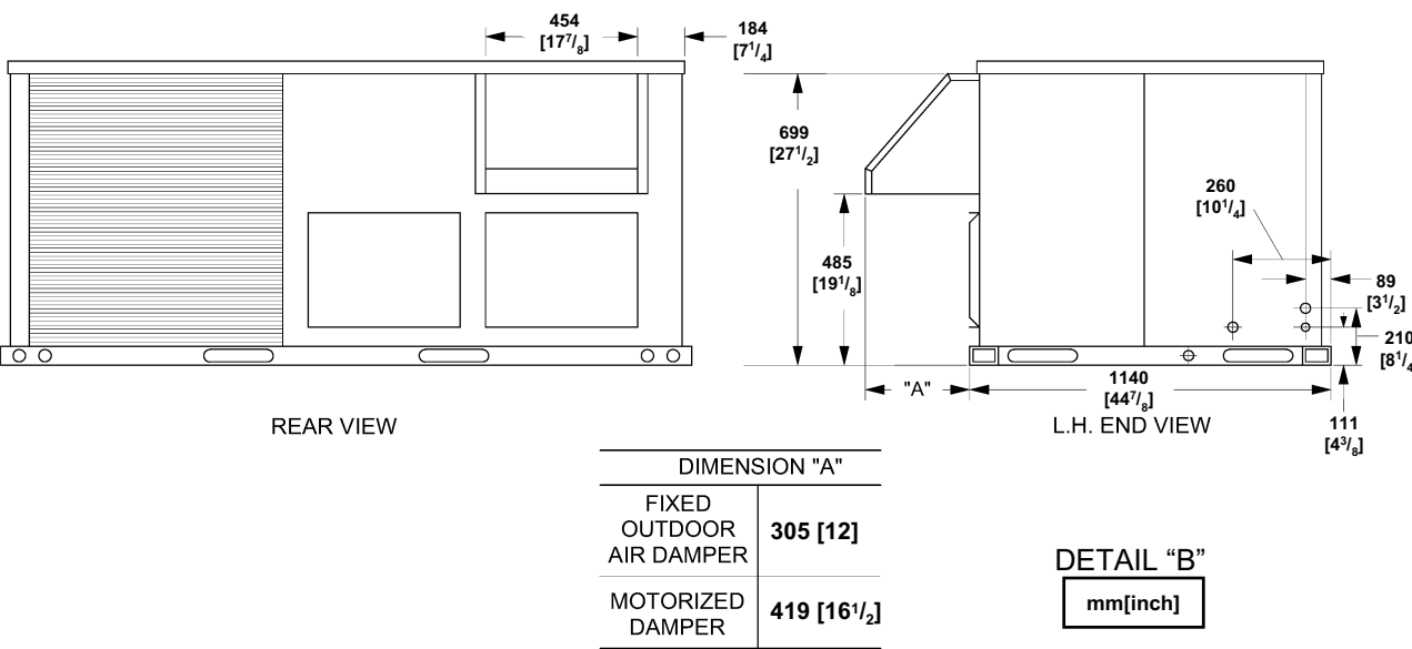
FIGURE 6 - UNIT WITH FIXED OUTDOOR AIR/MOTORIZED DAMPER RAINHOOD
