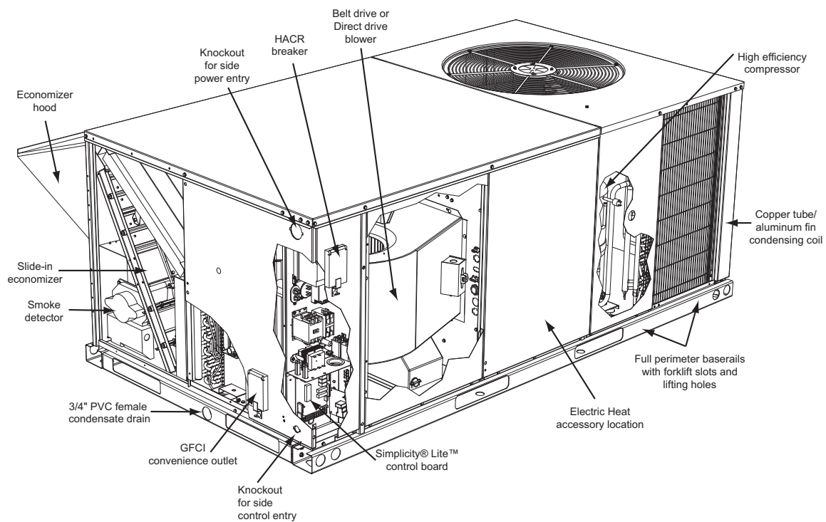
FIGURE 1 - UNIT CUTAWAY
