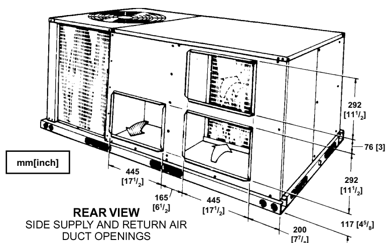
FIGURE 7 - UNIT DIMENSIONS (REAR VIEW)
